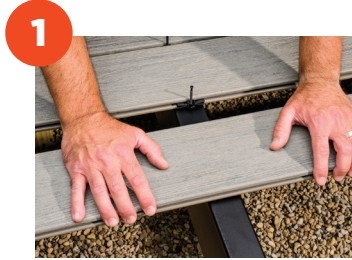
1 Lay rows of boards and CAMO EDGEXMETAL Clips down on the metal joists.
